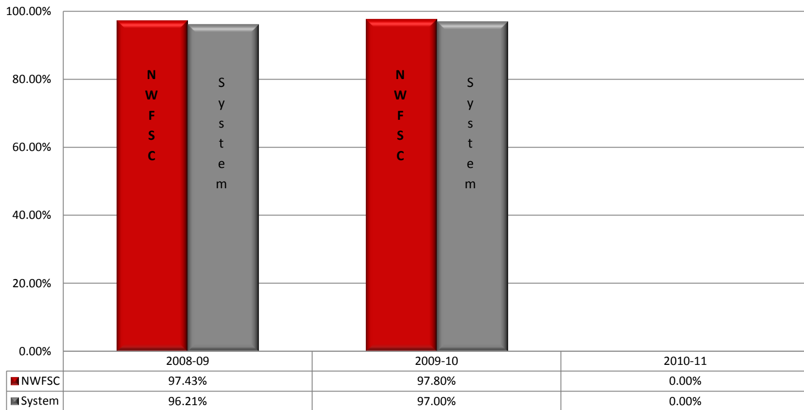
CLAST Performance
